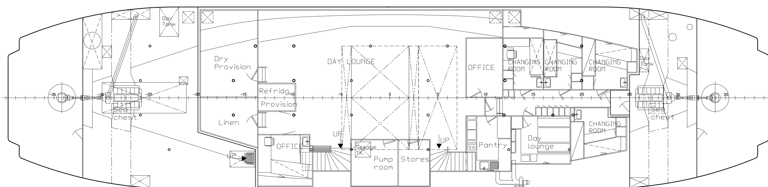
UNDER MAIN-DECK
