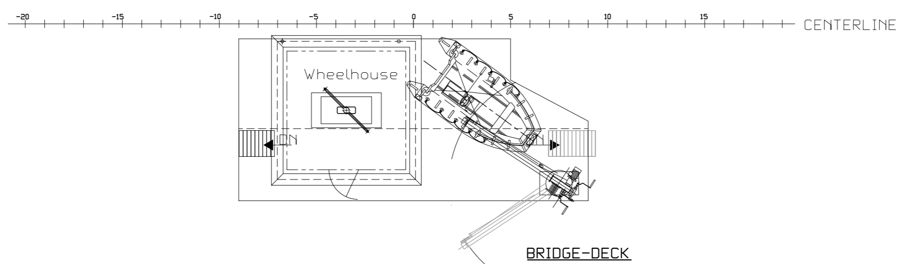
BRIDGE-DECK
