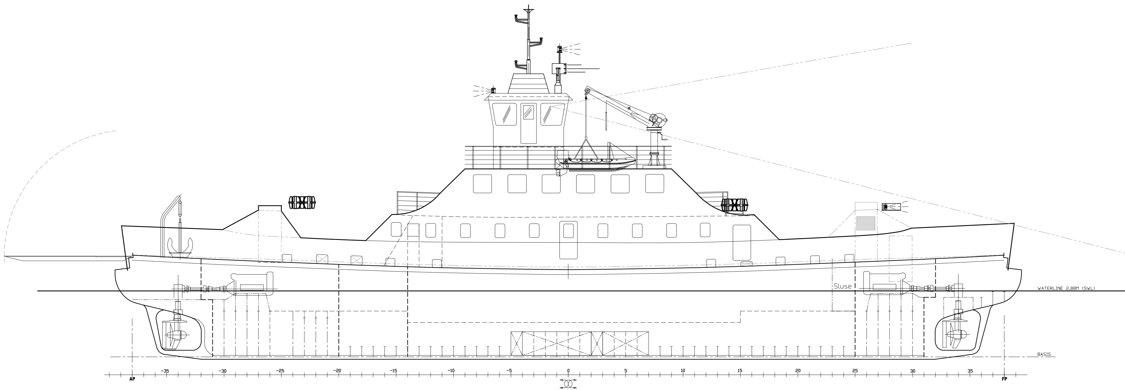
PROFILE
